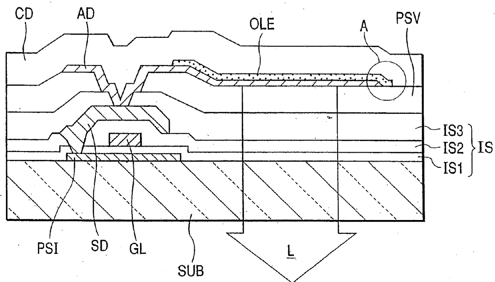
FIG. 15 (PRIOR ART)
