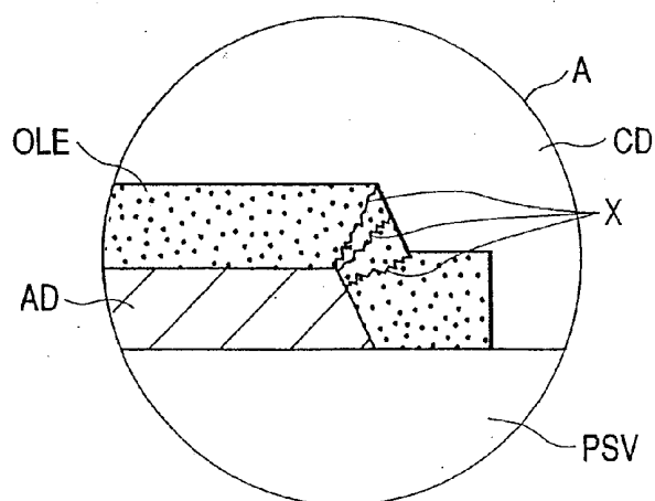
FIG. 16 (PRIOR ART)
